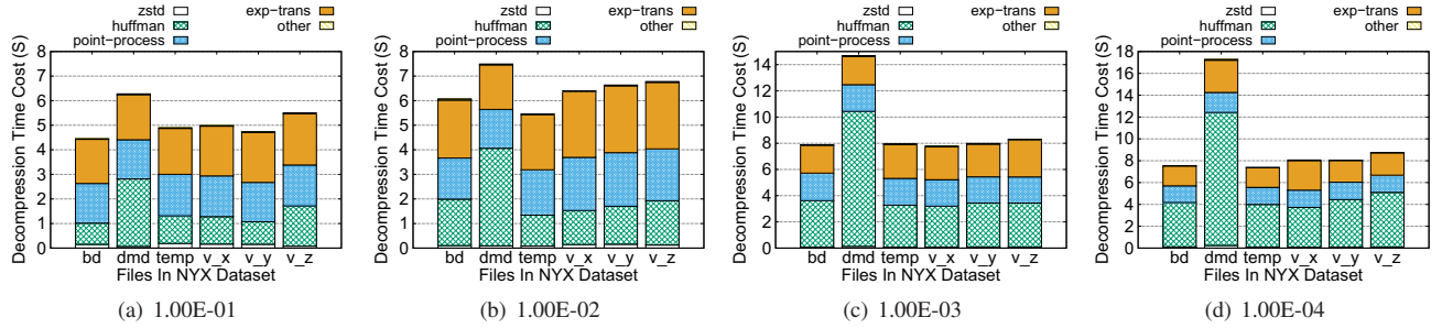
Fig. 3. Break-down of the decompression time for SZ with logarithmic transformation (using relative error bound on NYX dataset).
