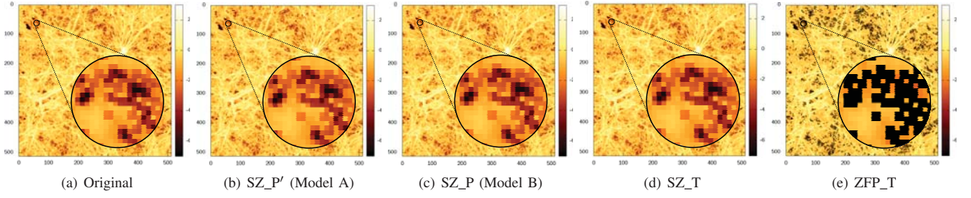
Fig. 13. Visualization of decompressed dark_matter_density dataset (slice 200) at the compression ratio of 2.75.
