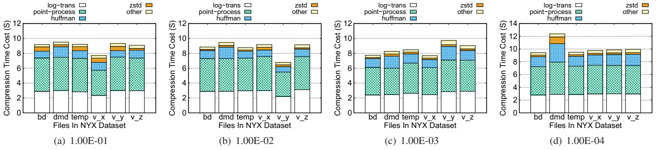
Fig. 2. Break-down of the compression time for SZ with logarithmic transformation (using relative error bound on NYX dataset).
