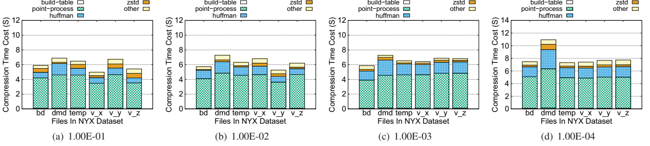
Fig. 10. Break-down of the compression time for SZ_P on NYX dataset.
