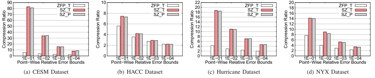
Fig. 12. Compression ratio on given point relative error bound.
