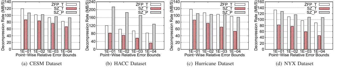
Fig. 9. Decompression rate on given point relative error bound.
