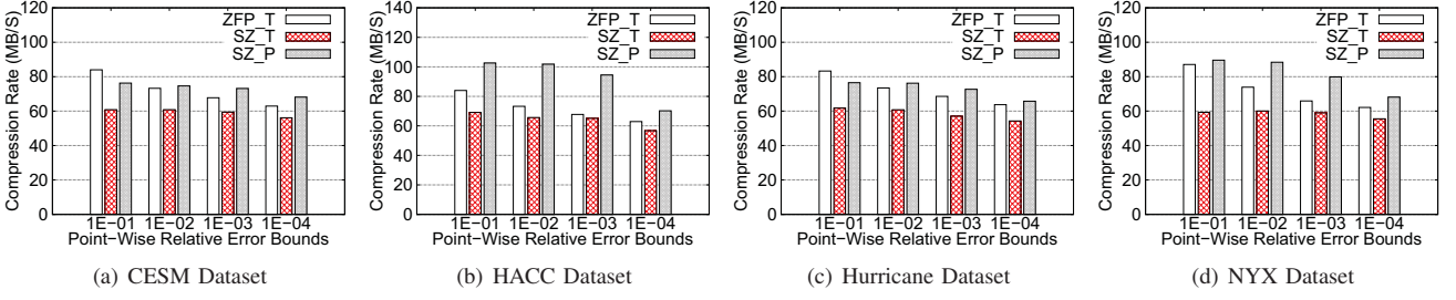
Fig. 8. Compression rate on given point relative error bound.
