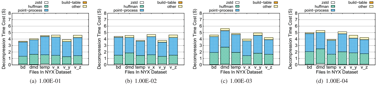
Fig. 11. Break-down of the decompression time for SZ_P on NYX dataset.
