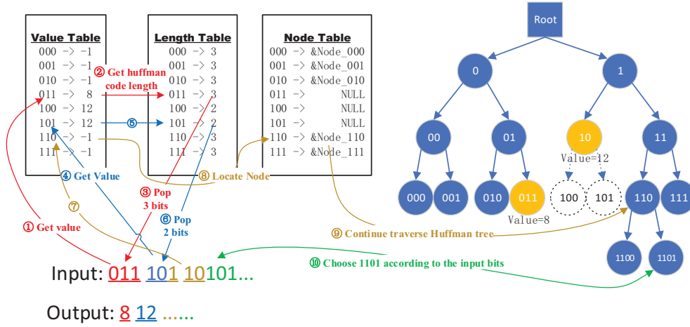
Fig. 7. An example of building precomputation-based tables to accelerate Huffman decoding in SZ_P.
