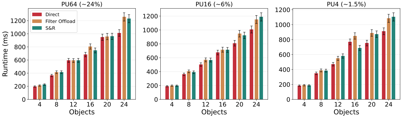
Fig. 8: Filter + group-by with varying selectivity. Left: PU = 64 (~24%). Center: PU = 16 (~6%). Right: PU = 4 (~1.5%).
